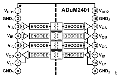
Figure 2. ADuM2401
